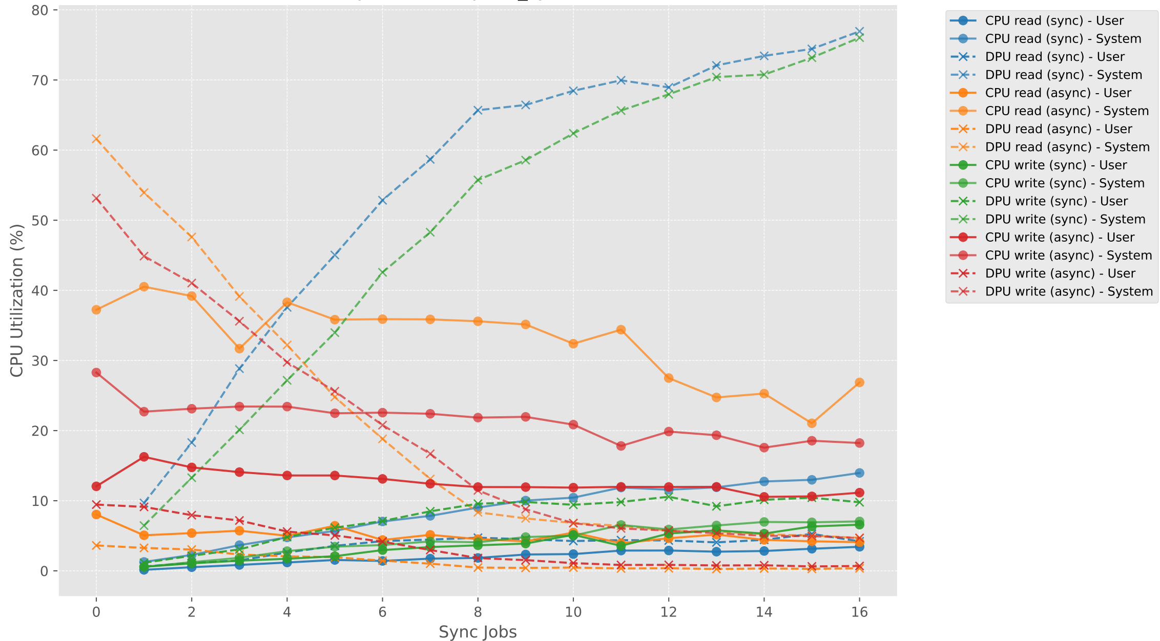
CPU Utilization vs Sync Jobs (async1_syncN)- SEQ (CPU vs DPU)
